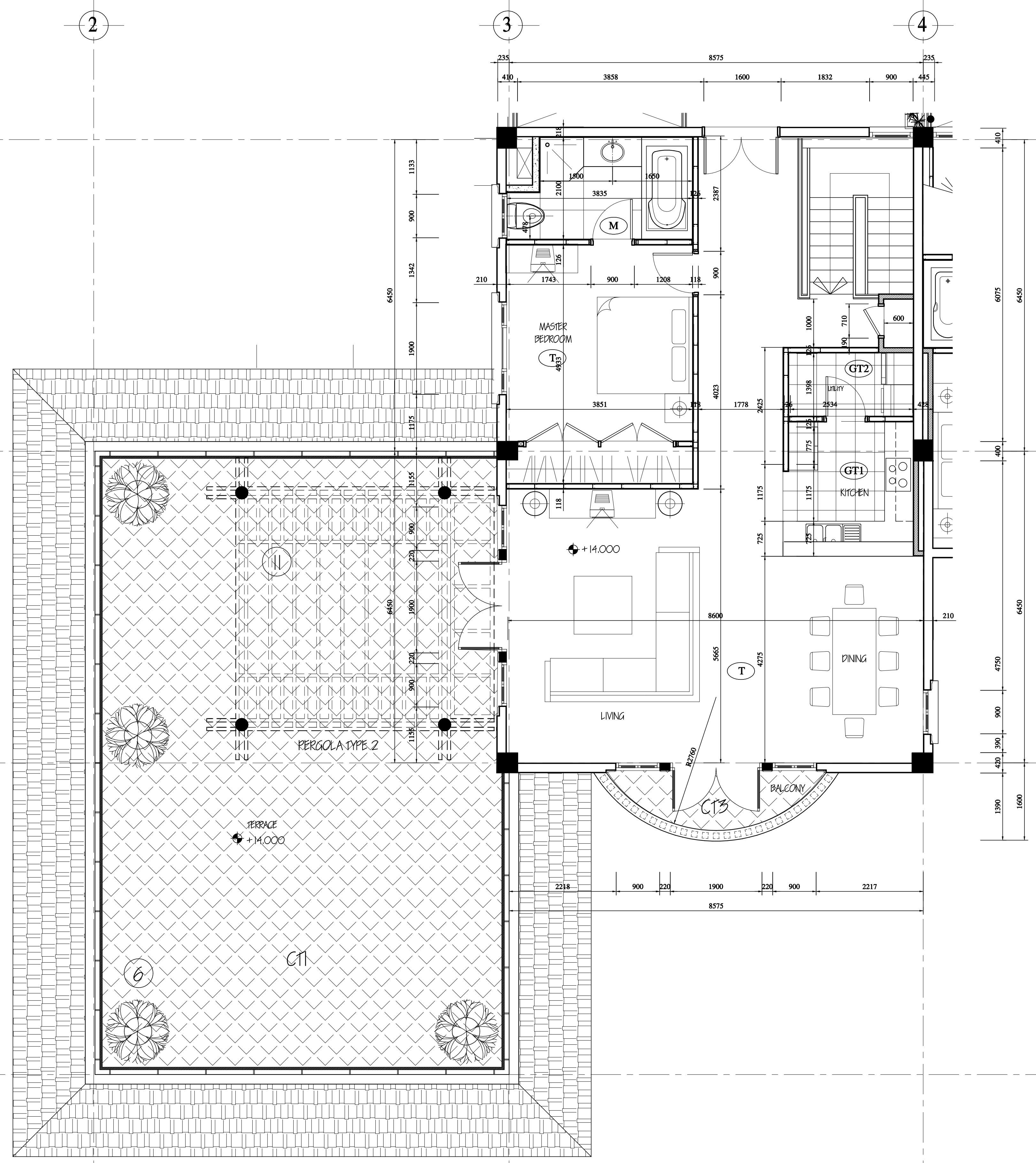
UPPER PART OF FLAT 30 SCALE: 1/50
