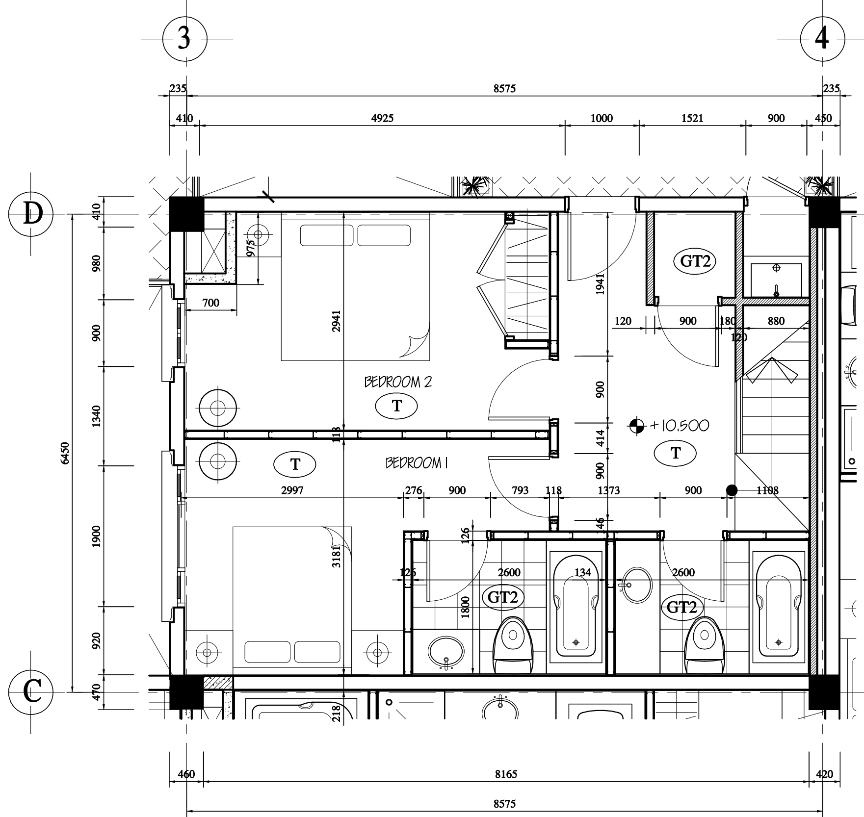
LOWER PART OF FLAT 30 SCALE: 1/50
