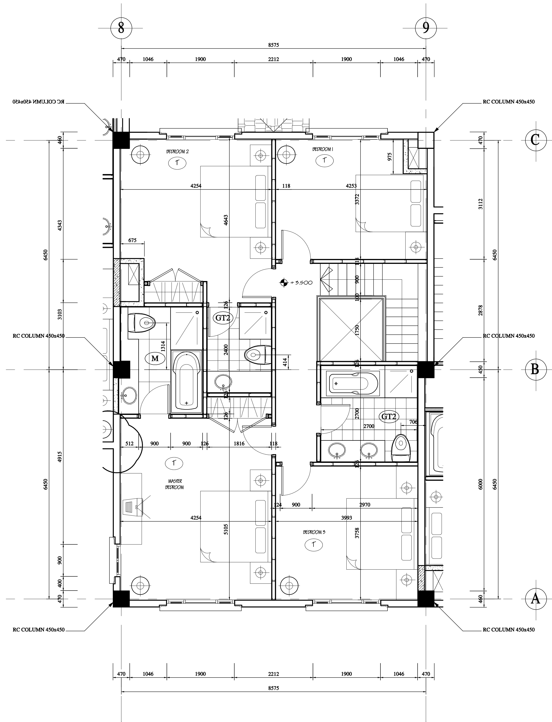
UPPER PART OF FLAT 13 SCALE: 1/50
